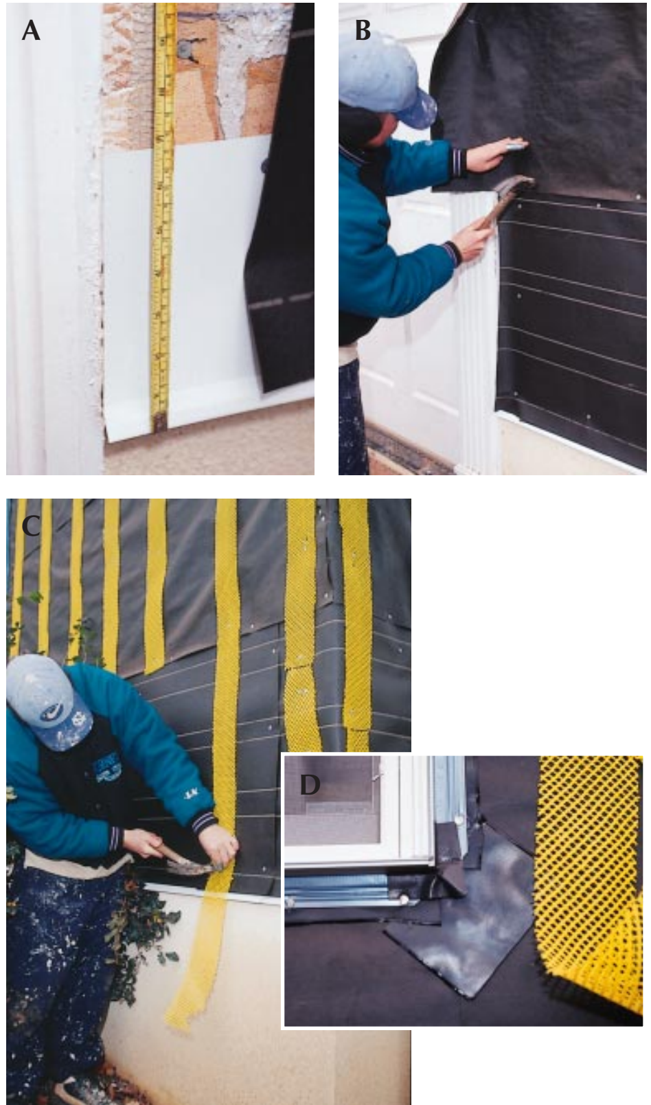
Figure 7. Installation of the drainage plane begins with vinyl or metal base flashing (A). The building is then wrapped in felt paper or Stuccowrap, with 4- to 6-inch overlaps at the joints (B), followed by staple-on mesh furring strips, which provide an air space behind the Durock (C). Extra care is taken to make windows and other openings watertight (D), using a self-sealing barrier tape where needed.
