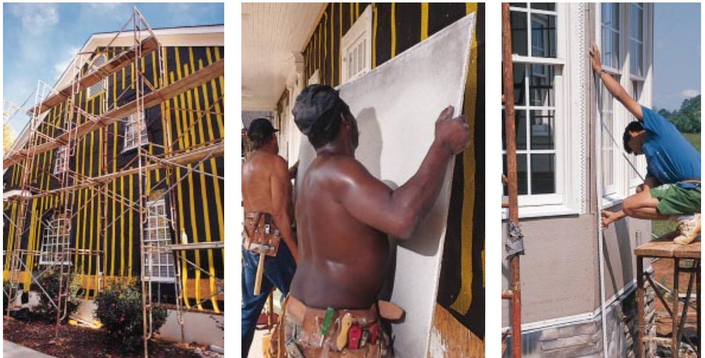
Figure 8. With the drainage plane and scaffolding in place (left), the Durock cement board panels are applied in a staggered pattern (middle). Spaces between panels provide a keyway for the stucco. A vinyl starter bead maintains a clean reveal along the exposed bottom edge of the cement board (right).
