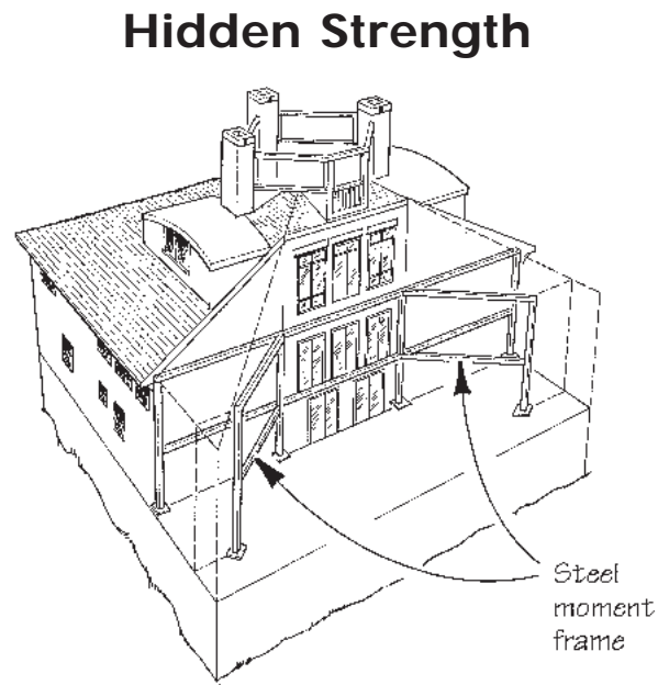
Figure 1. The expanse of windows walls in the east wall of this oceanfront home leaves no room for plywood shear walls (left). A structural steel moment frame embedded in the framing (right) handles large lateral wind loads.
